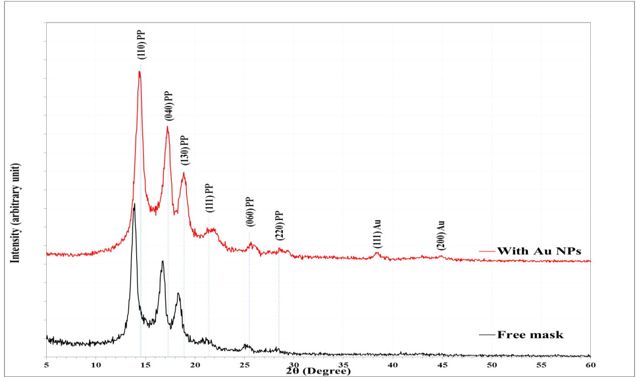
Figure 2. XRD patterns for pure mask and decorated samples with Au NPs.
