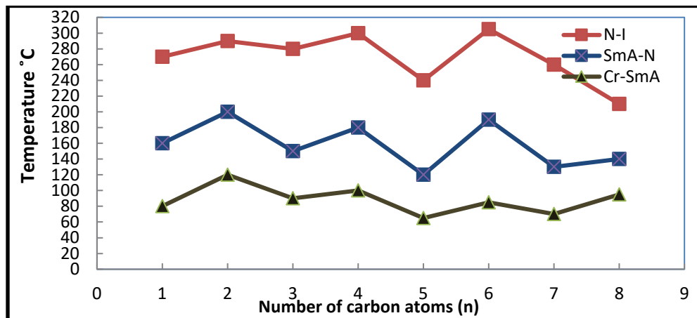
Figure 2. A graph of the transition temperature against the number of carbon atoms (n) in the [V]n alkoxy chain series.
