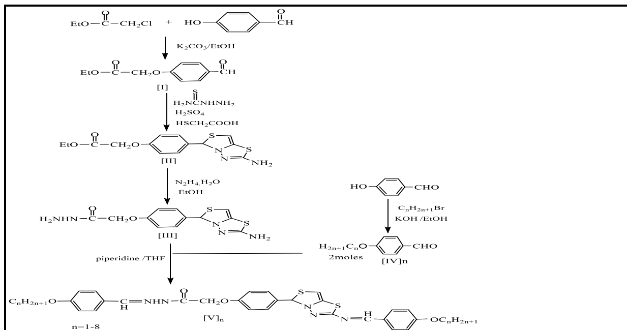
Scheme 1. Route of synthesis compounds [I]-[V]8.
