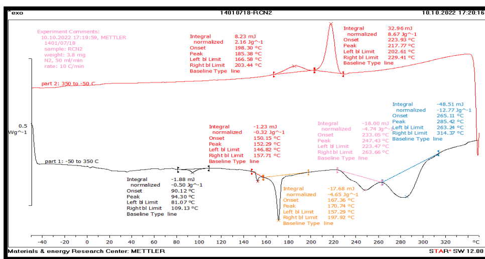
Figure 3. The DSC thermogram for compound [V]2.
