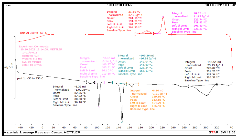
Figure 4. The DSC thermogram for compound [V]7.
