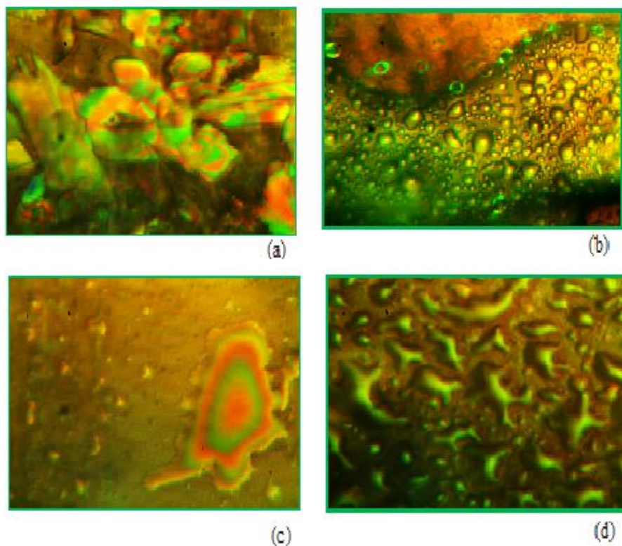
Figure 1. Cross polarizing optical textures of (a) smectic A phase for compound [V] 2 at 220 °C (b) droplets nematic phase for compound [V] 3 at 275 °C (c) nematic phase for compound [V] 6 at 300 °C (d) nematic phase for compound [V] 7 at 295 °C.
