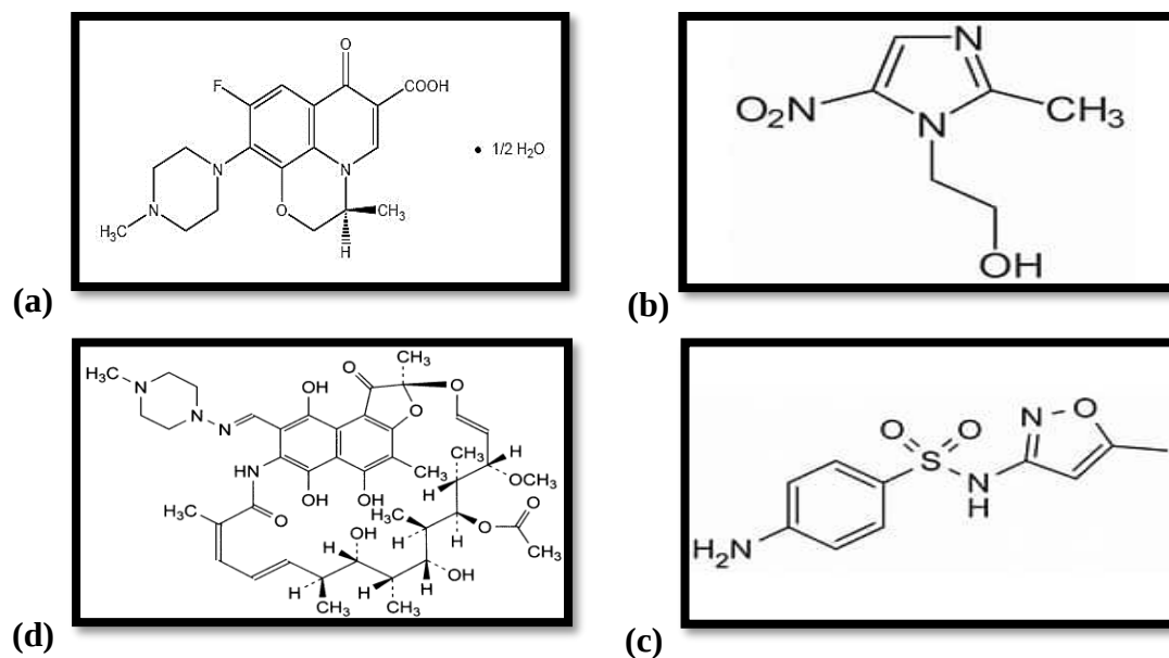
Figure 1. Structures formula of (a) Levofloxacin, (b) Sulfamethoxazole, (c) Metronidazole and (d) Rifampicin.
