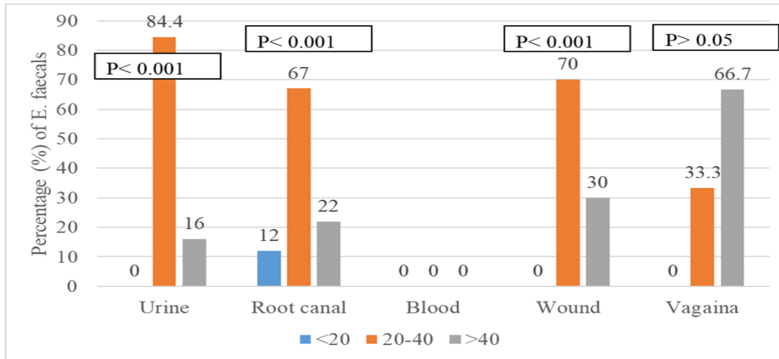
Figure 1. The prevalence of E. faecalis according to the age.
