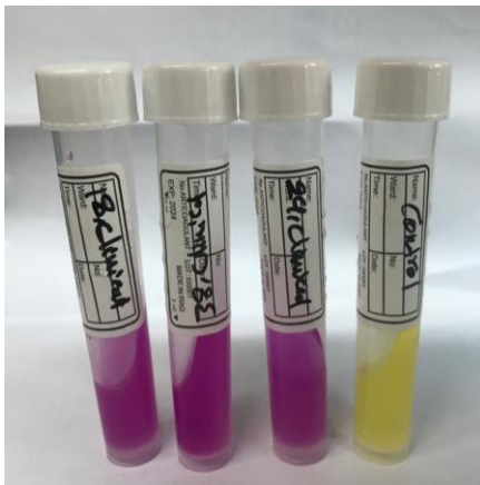
Figure 4. Proteus inoculated into Christensen medium which give positive results pink color after 24h of incubation at 37°C.
