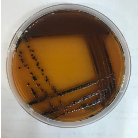
Figure 2. Proteus mirabilis on Salmonella Shigella agar after 24h of incubation at 37°C, the colonies appear pale with black center (hydrogen sulfide production).
