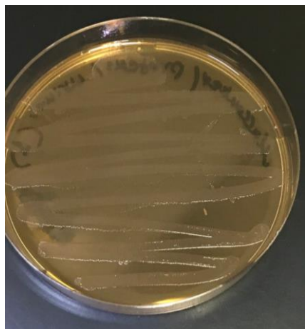
Figure 1. Proteus mirabilis on MacConkey agar after 18- 24h of incubation at 37°C, the colonies appear as smooth and pale colonies.
