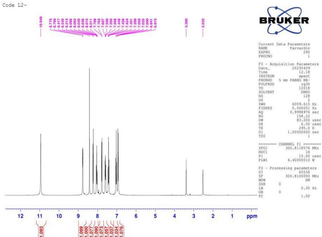
Figure 13. The ^1\text{H} -NMR of ligand L 2 .
