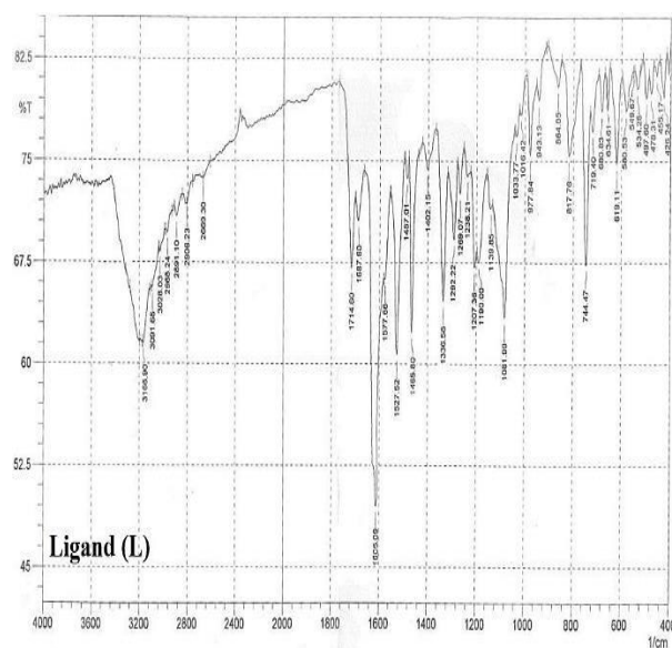
Figure 7. The FTIR-spectrum of L.
