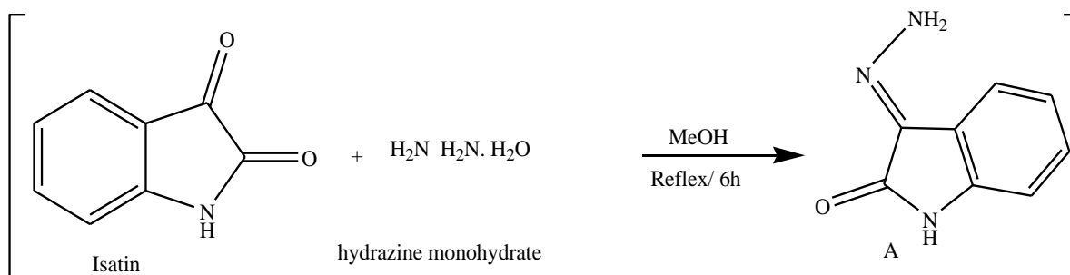
Scheme 1. Preparation of the (A) basic material.
