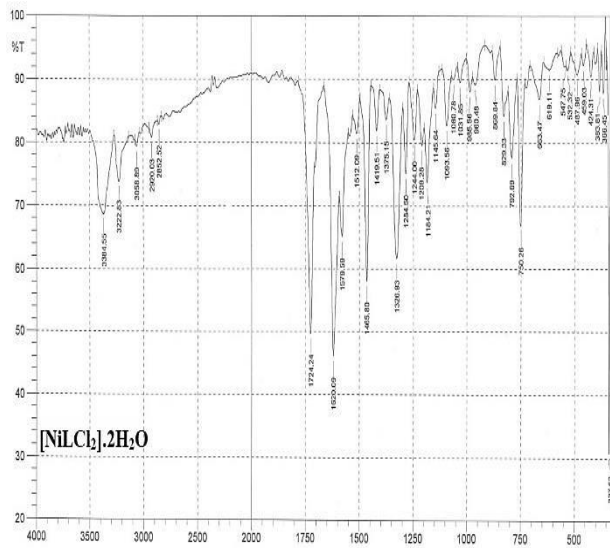
Figure 10. The FTIR-spectrum of Ni L complex.
