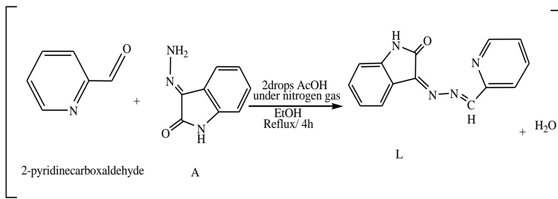
Scheme 2. The prepared of Schiff bases ligand.
