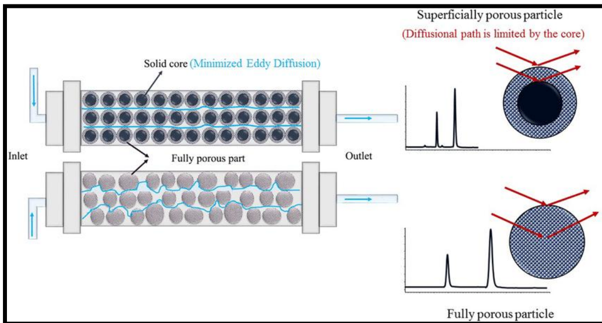
Figure 2. The contrast between fully porous particle distribution (traditional silica) and narrow particle distribution (superficial silica) is an example of the impact on peak efficiency and analysis time.
