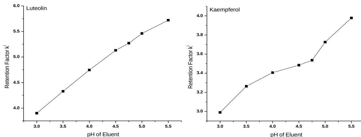
Figure 6. Effect of pH on the behavior of kaempferol and luteolin using a HALO-HILIC.
