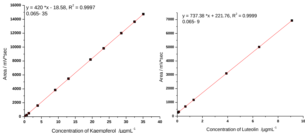
Figure 7. Calibration curves of standard solutions of kaempferol and luteolin.
