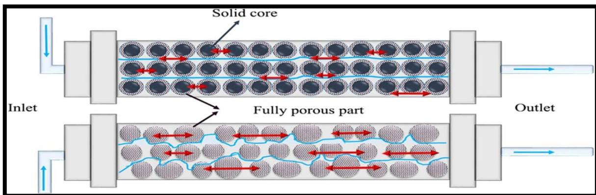
Figure 3. An illustration of the effect of the B term is provided by solid core particles preventing diffusion as a solute diffuses through a pore and outside of totally porous particles.
