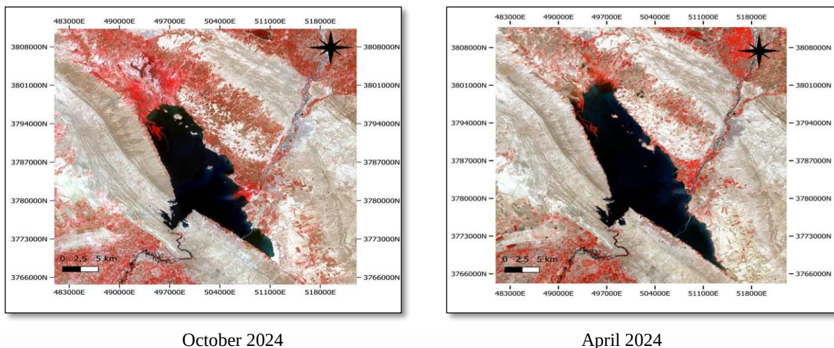
Figure 2. Satellite images of the lake Hamrin for two seasons "EPSG:32638-WGS84/UTM Zone 38"
