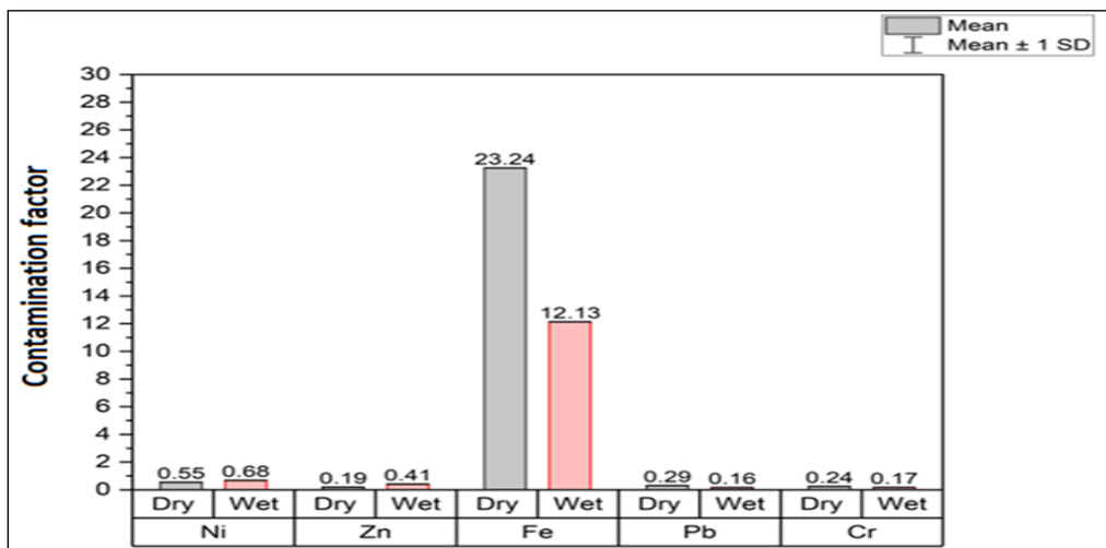
Figure. 6. Contamination Factor (Cf) of heavy metals in Tigris River sediments during dry and wet seasons (mean ± SD).
