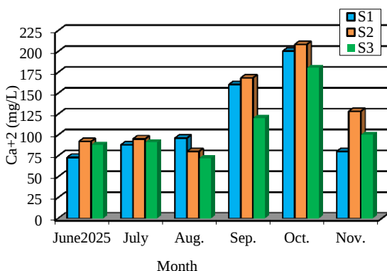
Figure 11. Variation of \text{Ca}^{+2}
