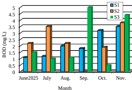
Figure 8. Variation of BOD
