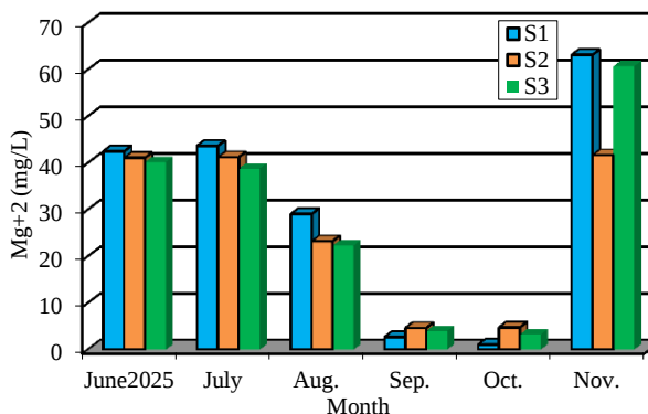
Figure 12. Variation of \text{Mg}^{+2}
